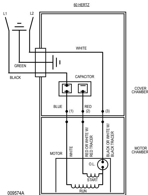
WIRING DIAGRAM FOR MODELS "N140" All Revisions; "N4140" All Revisions; "E140" All Revisions; "E4140" All Revisions 2/95 thru Current
